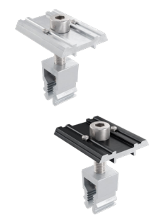
middle 30-35 clamp uni ic 50 with pin / mittelklemme 30-35 uni ik 50 pin material: EN AW-6063 T66 / A2-70
