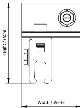
Winkel 60 mm, M10 Bracket 60 mm, M10
