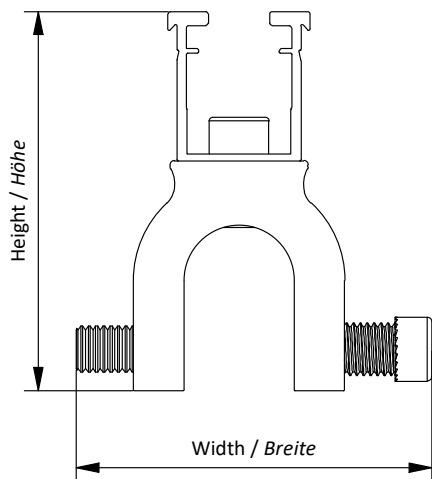
rundfalzklemme bk uni circular seam clamp bk uni
