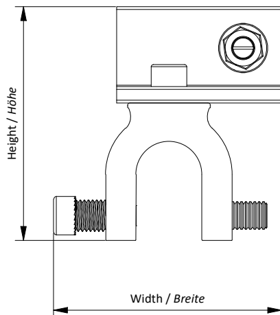
rundfalzklemme bw uni circular seam clamp bw uni
