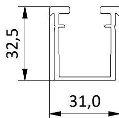
Trapezblechkurzschiene 35 Uni Trapezoidal short rail 35 Uni
